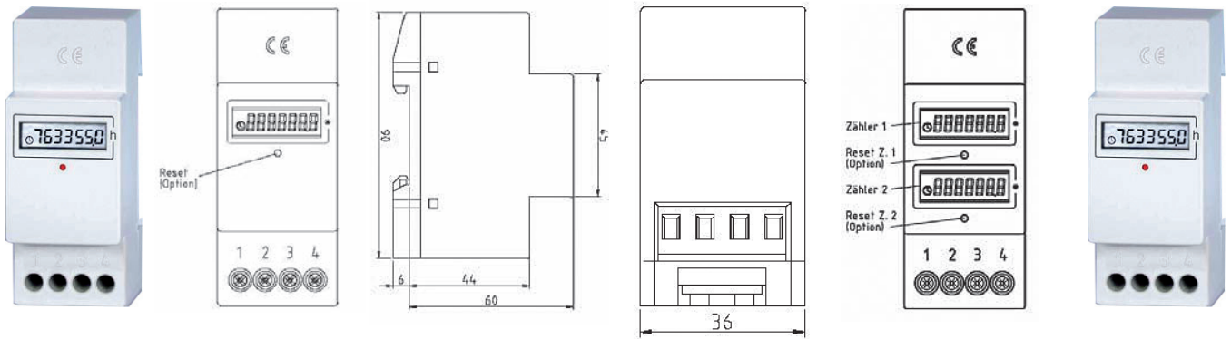
670.6...36 mm = 2TE
